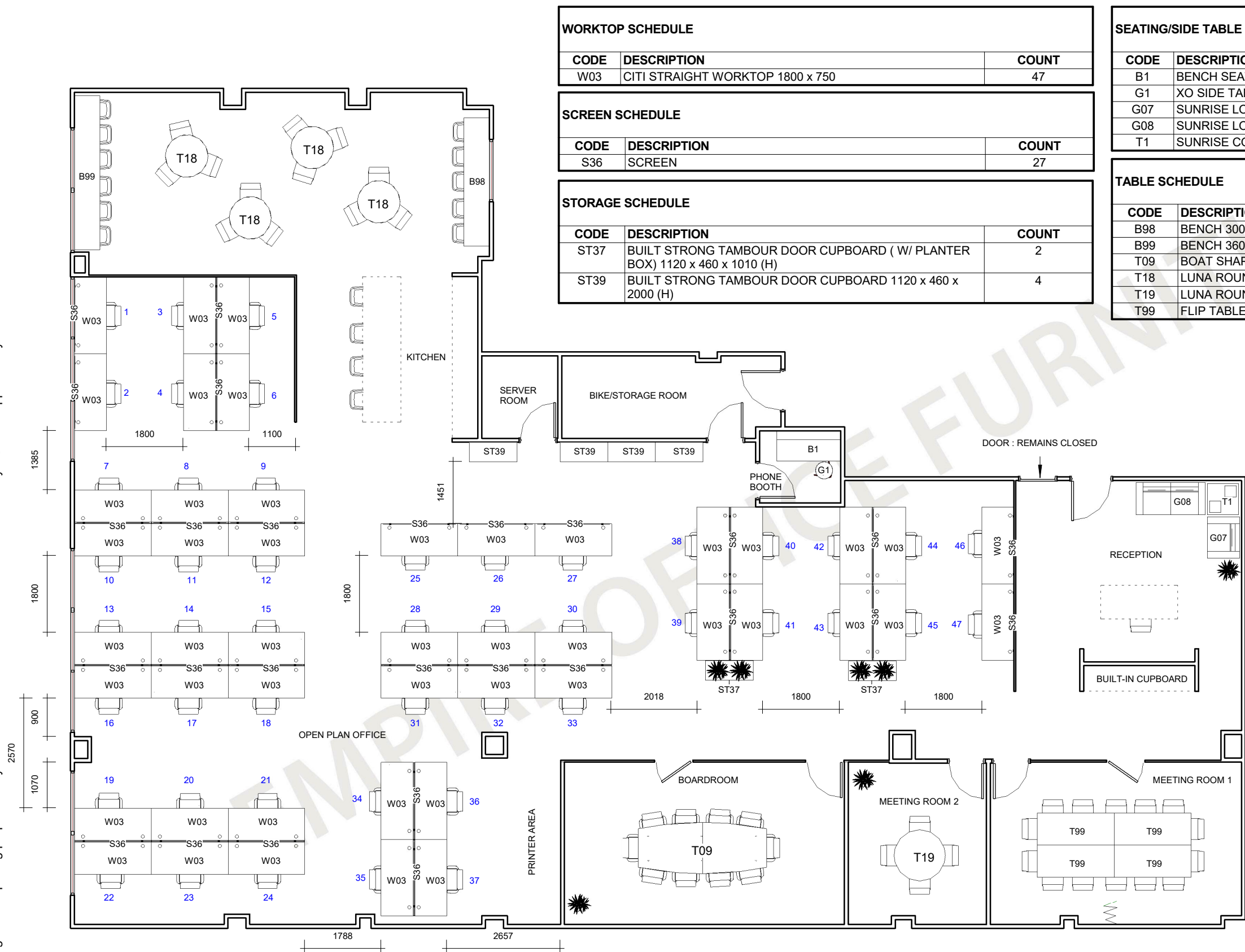
1 WORKSTATION LAYOUT 1 : 100
